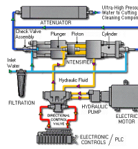
pumping system
