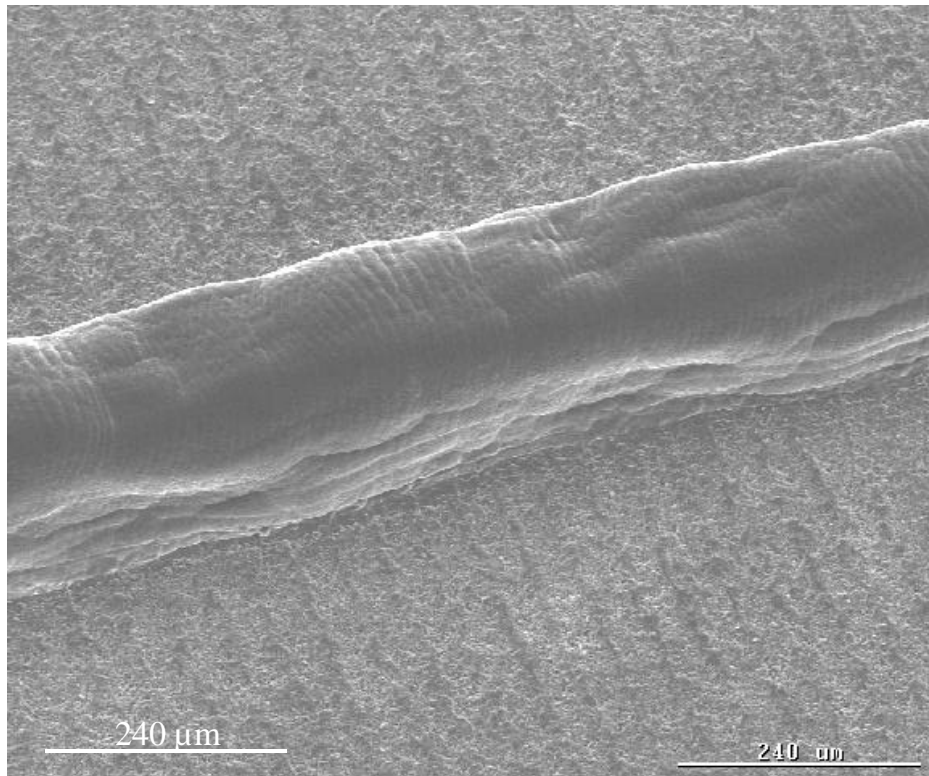
Figure 4. Twenty pass wall deposited using temperature control. 7
