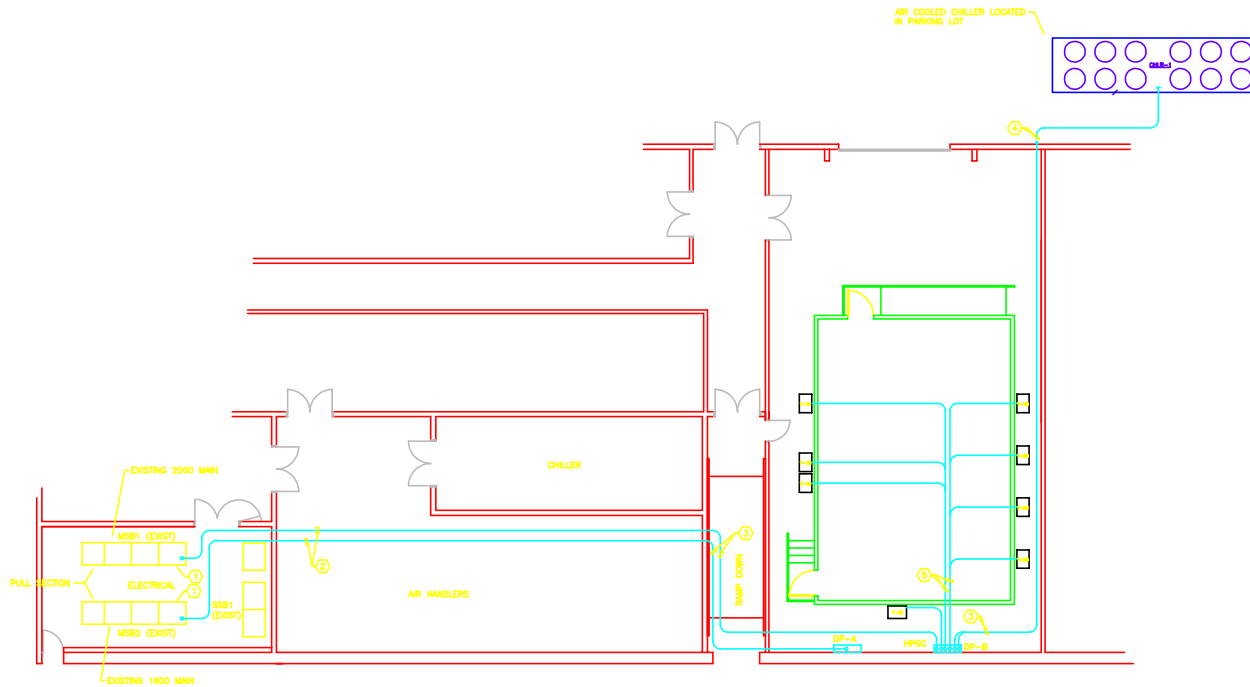
① POWER ROUTING PLAN SCALE: 1/8" = 1'-0"
