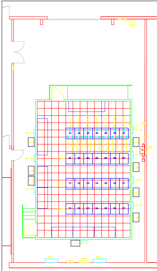
1 POWER PLAN SCALE: 1/4" = 1'-0"
