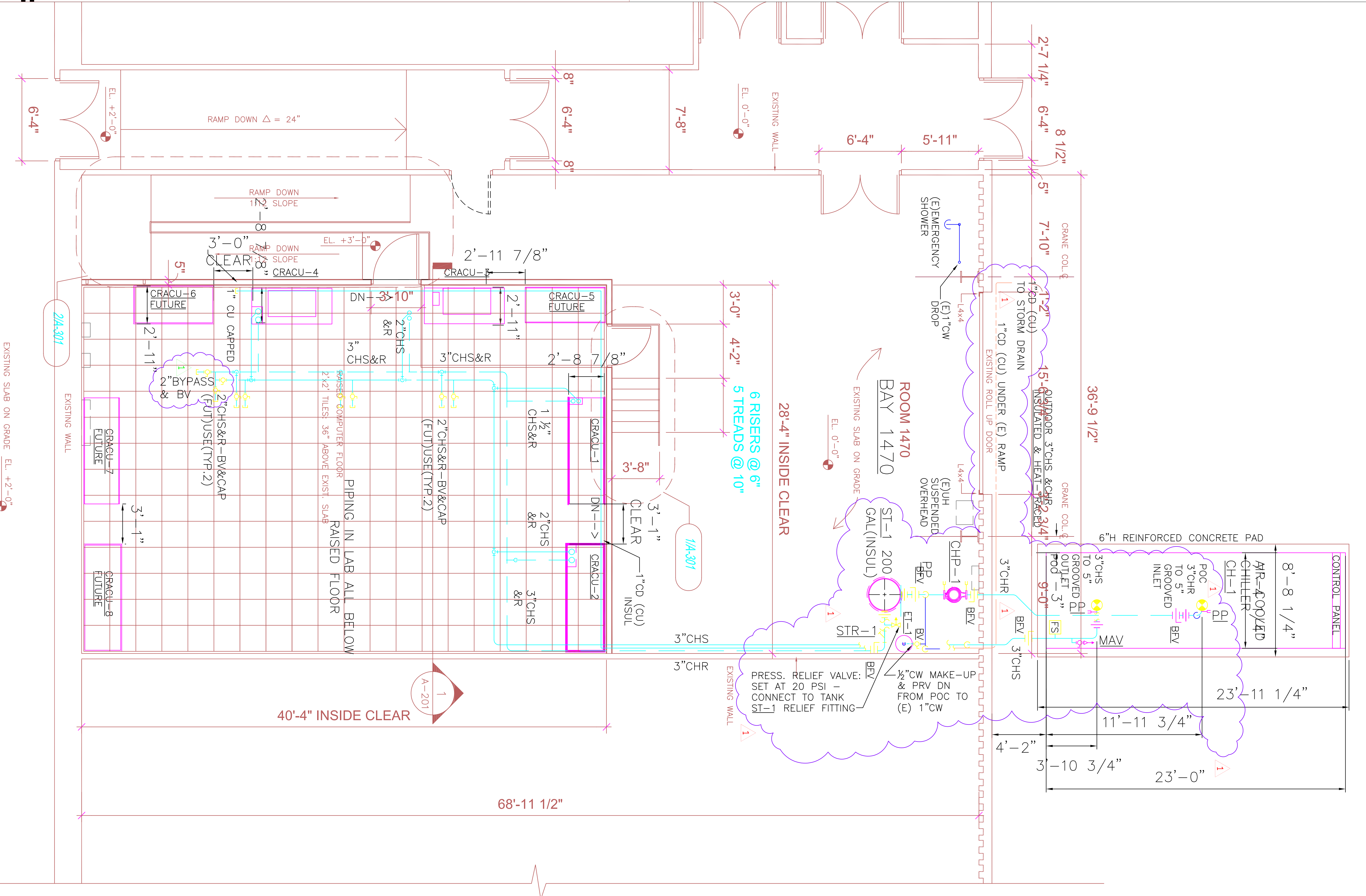
1 DATA LAB PIPING PLAN SCALE: 1/4"=1'-0"
