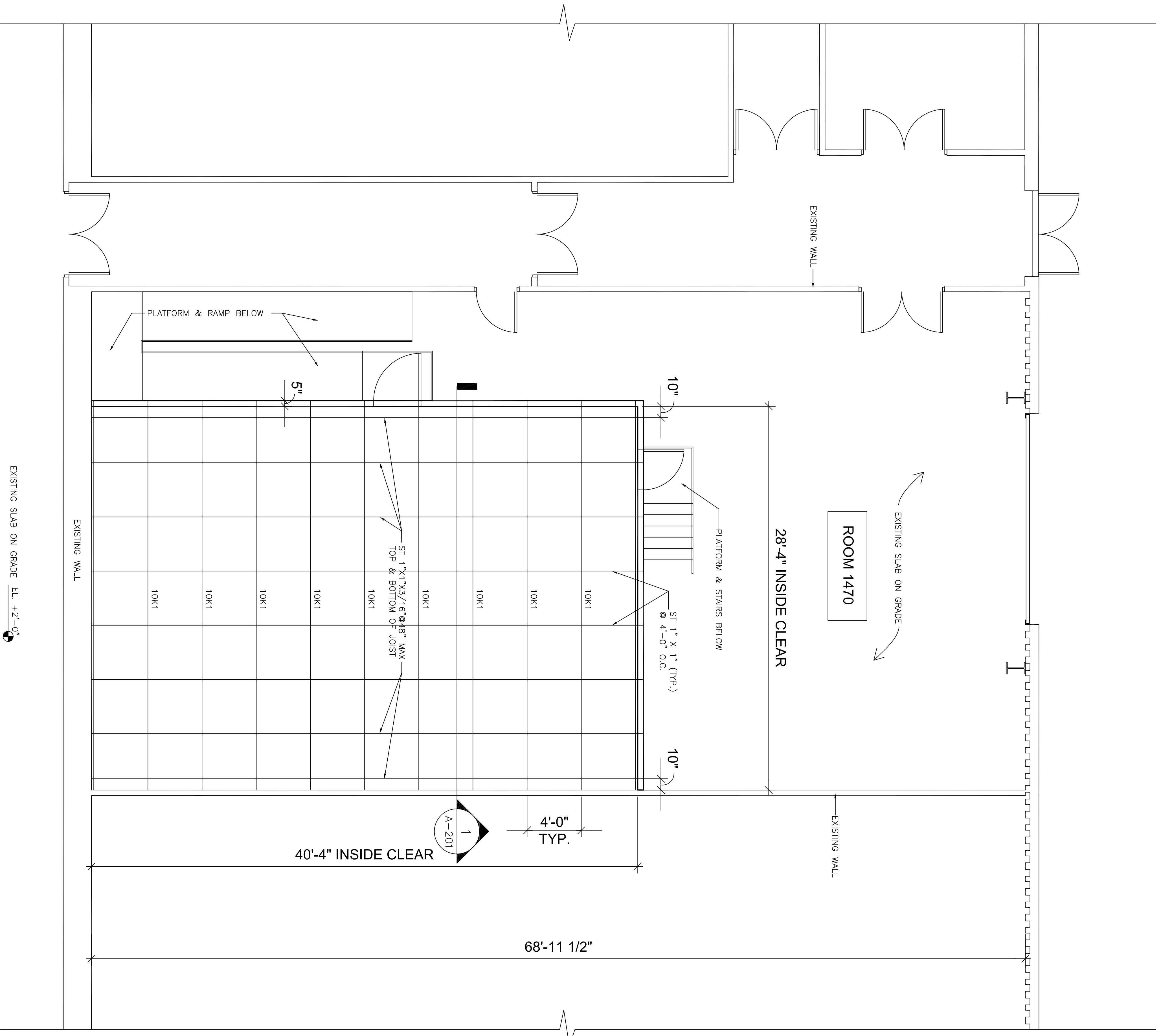
1 PLAN: SUPPORT LEVEL FOR HVAC / CEILING SYSTEMS (DATA CENTER) HATCHING SCALE: 1/4" = 1'-0"
