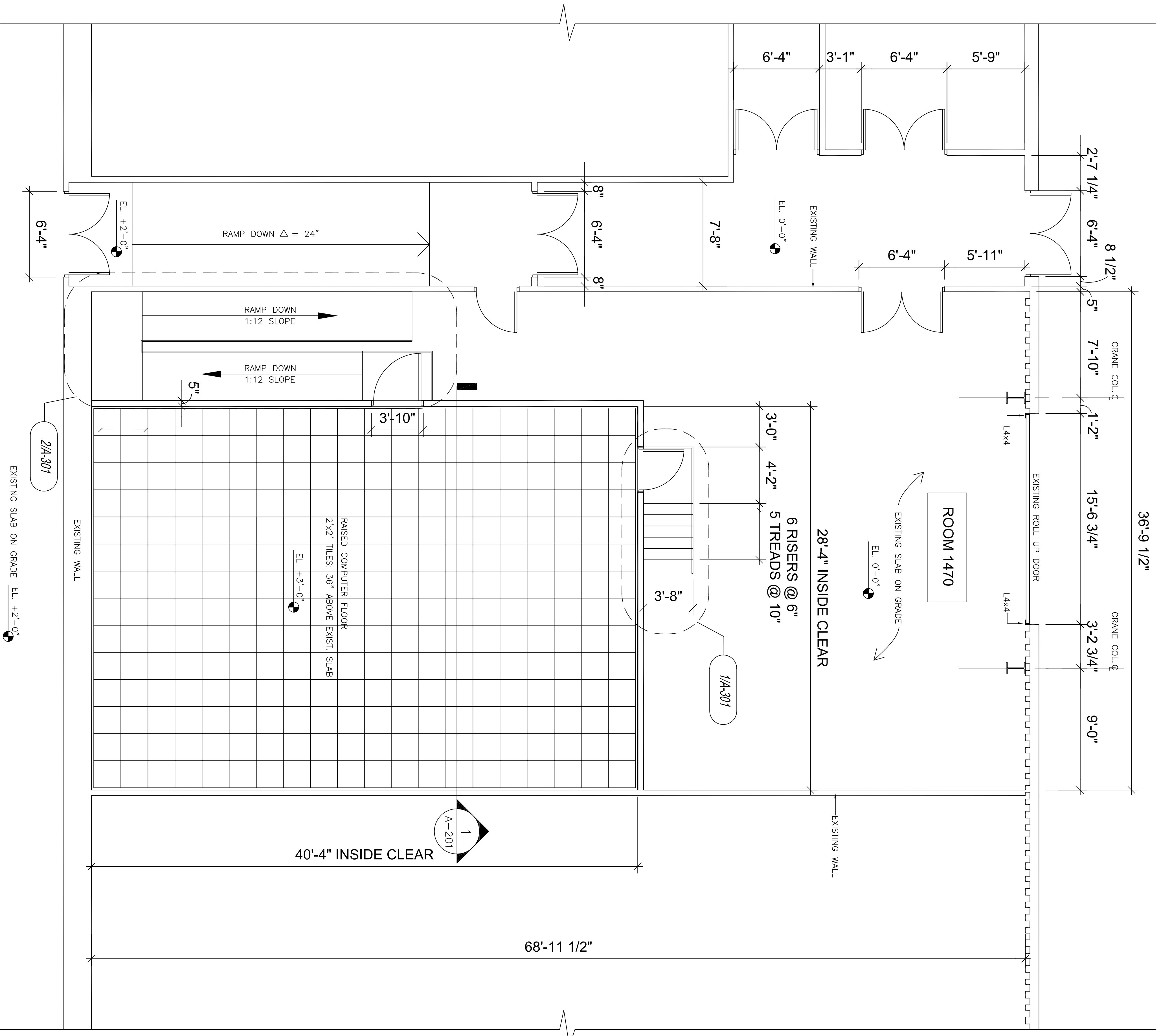
1 PLAN: DATA CENTER LAB FACILITY / ROOM 1470 HORIZONTAL SCALE: 1/4" = 1'-0"
